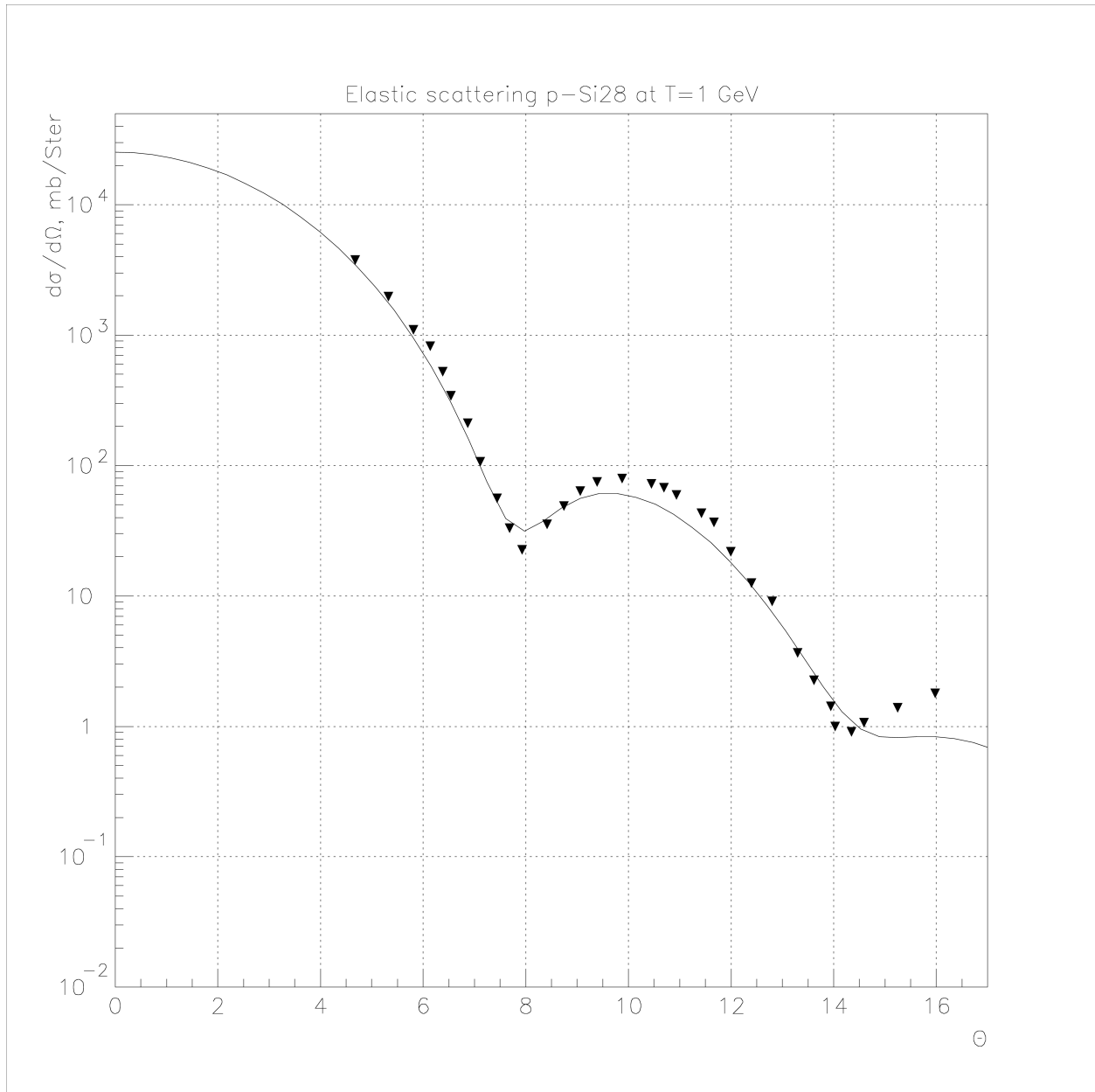
Fig. 21.5: Elastic proton scattering on ^{28}\text{Si} at 1 GeV.
