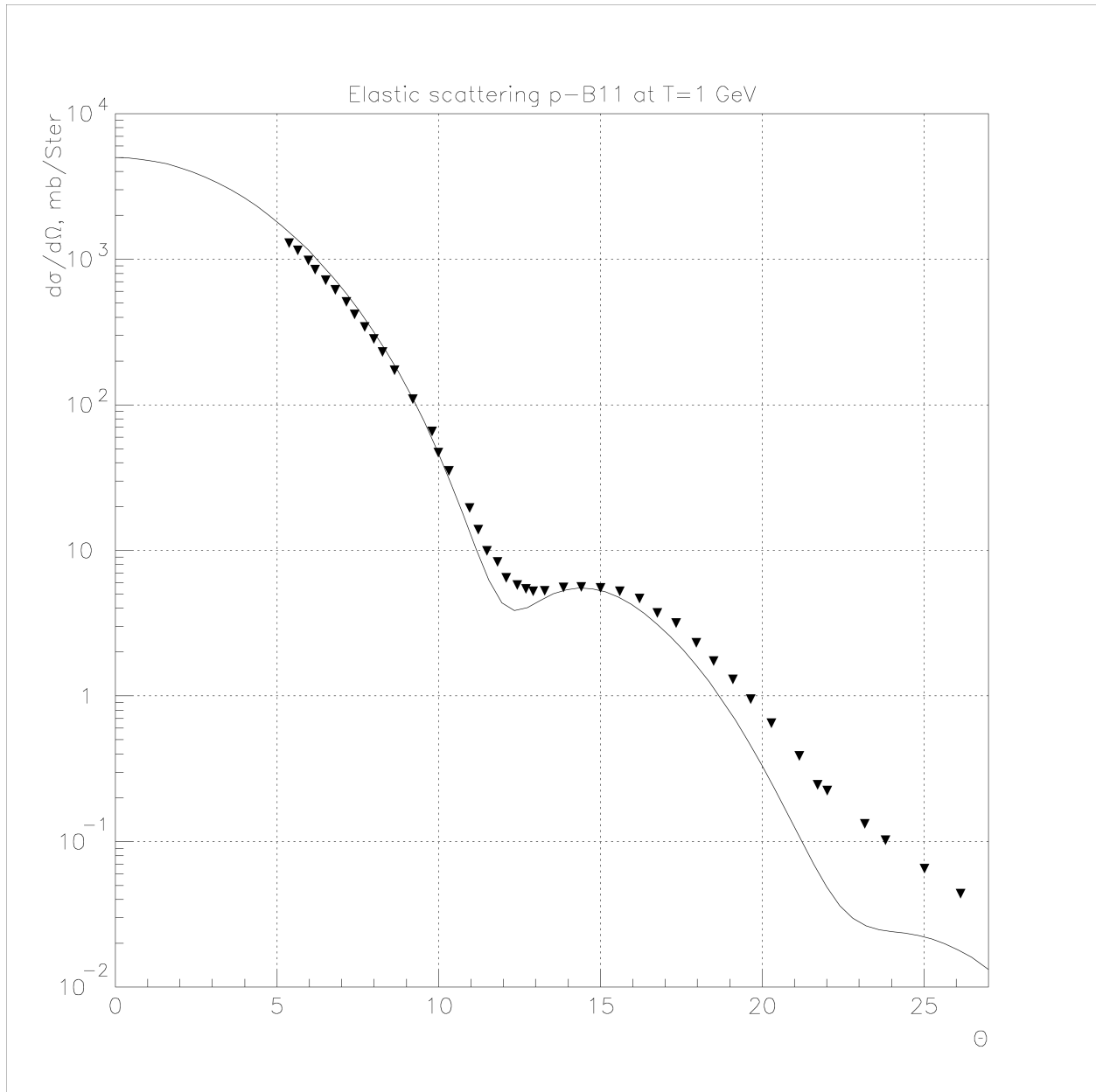
Fig. 21.2: Elastic proton scattering on ^{11}\text{B} at 1 GeV.
