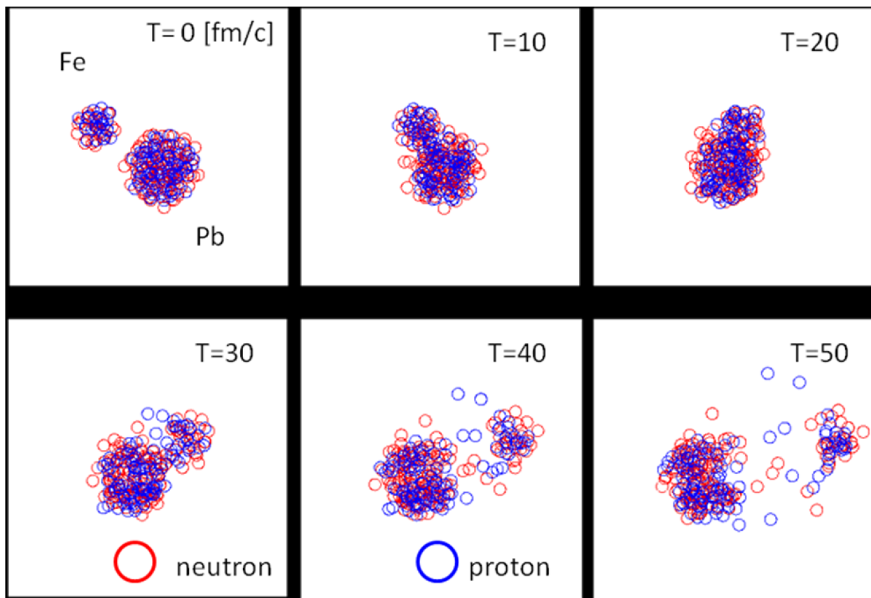
Fig. 33.1: Time evolution of reaction of 290 MeV/n Fe on Pb in position space. Red and Blue circle represents neutron and proton respectively. Full scale of each panel is 50 fm.
