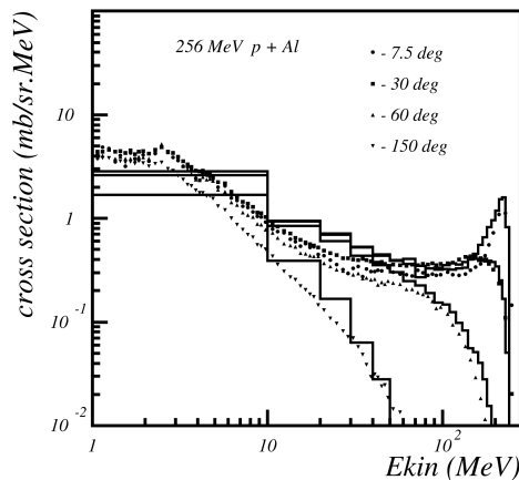
Fig. 25.2: Double differential cross-section for neutrons produced in proton scattering off Aluminum. Proton incident energy was 256 MeV. The points are data, the histogram is Binary Cascade prediction.
