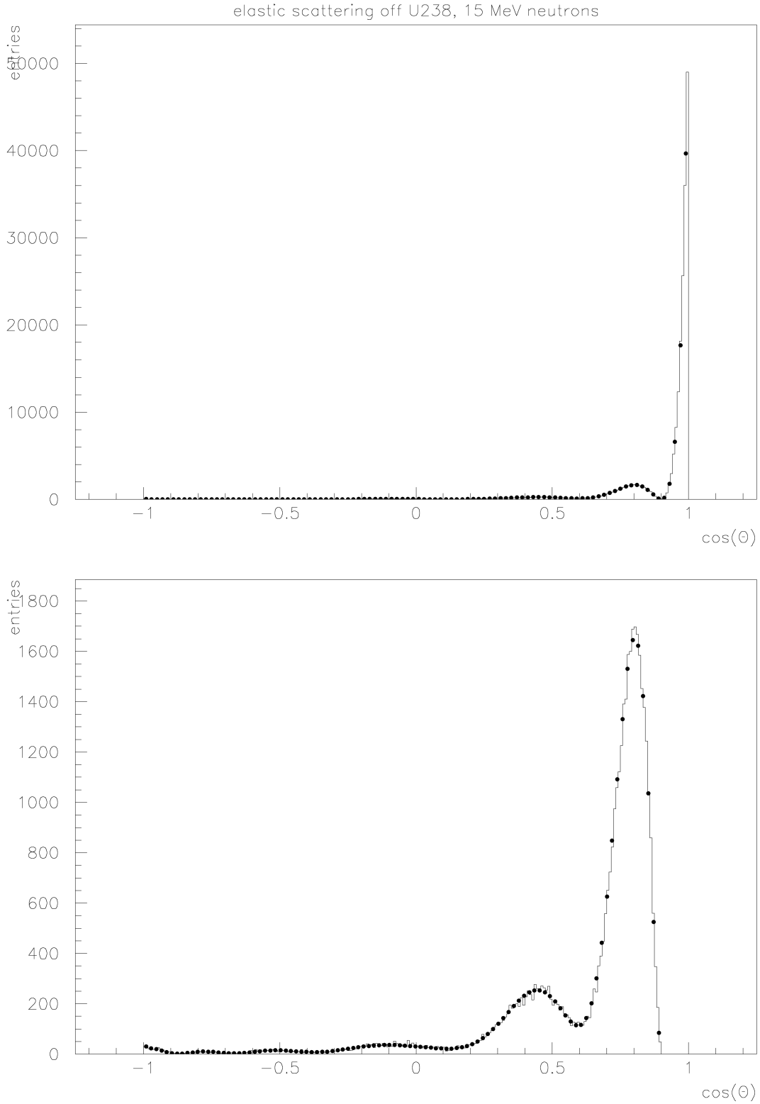
Fig. 37.1: Comparison of data and Monte Carlo for the angular distribution of 15 MeV neutrons scattered elastically off uranium ( ^{238}\text{U} ). The points are evaluated data, and the histogram is the Monte Carlo prediction. The lower plot excludes the forward peak, to better show the Frenel structure of the angular distribution of the scattered neutron.
