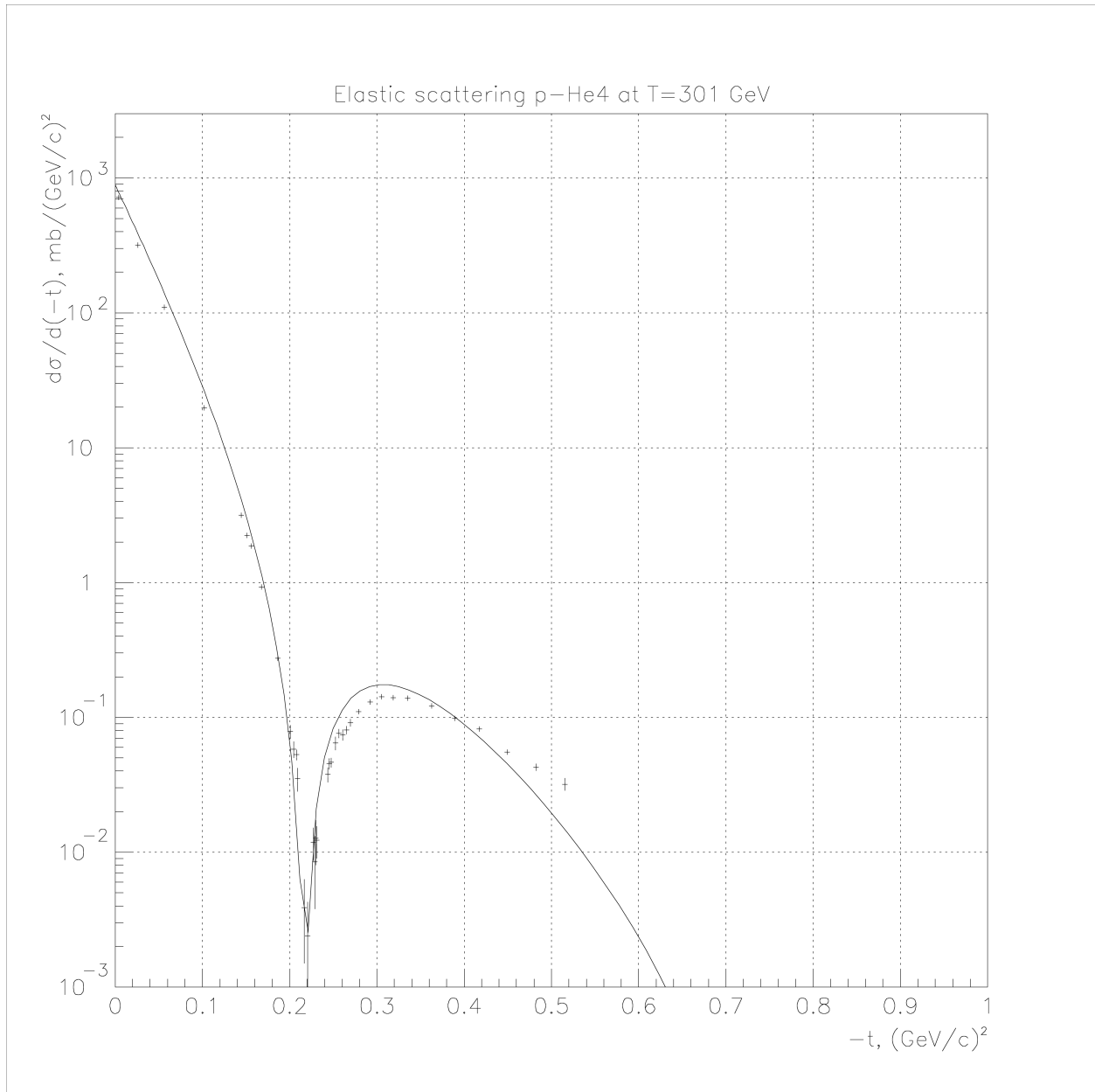
Fig. 21.12: Elastic proton scattering on ^4\text{He} at 301 GeV.
