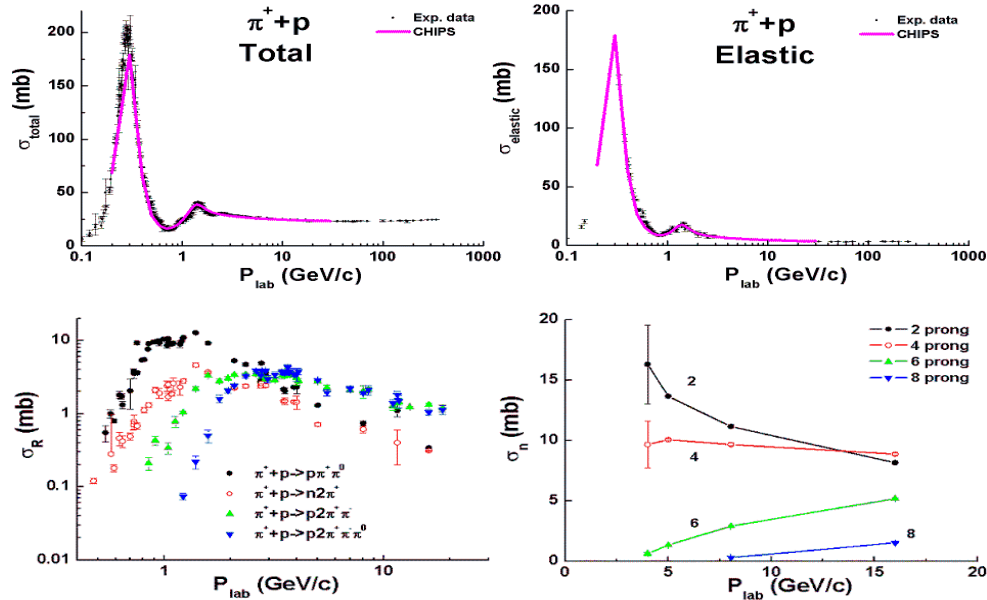
Fig. 23.5: General properties of \pi^+p -interactions. Points are experimental data: data on total and elastic cross sections from PDG data-base [PDG12], other data from [eal72].
