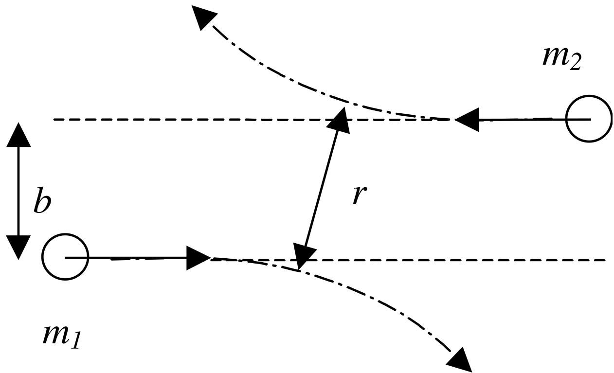
Fig. 34.2: Illustration clarifying impact parameter in the far-field ( b ) and actual impact parameter ( r ).
