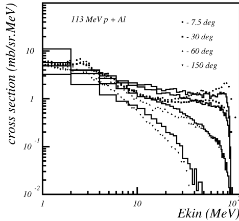
Fig. 25.1: Double differential cross-section for neutrons produced in proton scattering off Aluminum. Proton incident energy was 113 MeV.
