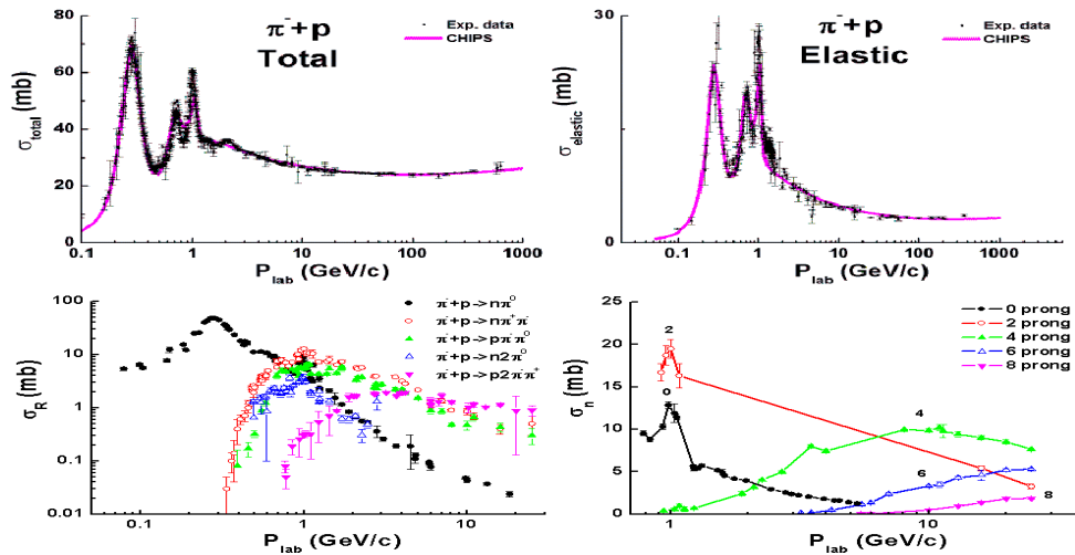
Fig. 23.3: General properties of \pi^-p -interactions. Points are experimental data: data on total and elastic cross sections from PDG data-base [PDG12], other data from [eal72].
