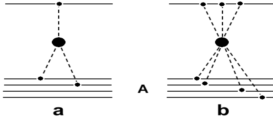
Fig. 23.18: Possible enhanced diagrams of hA -interactions.
