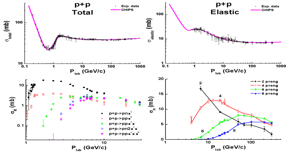
Fig. 23.6: General properties of pp -interactions. Points are experimental data: data on total and elastic cross sections from PDG data-base [PDG12], other data from [eal73a, eal84].
