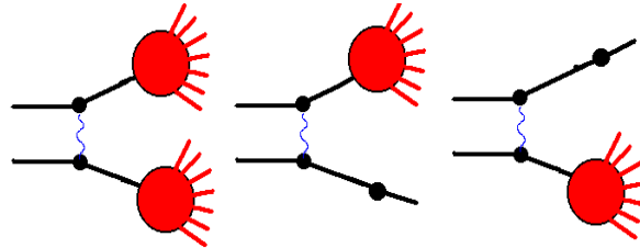
Fig. 23.1: Non-diffractive and diffractive interactions considered in the Fritiof model.
