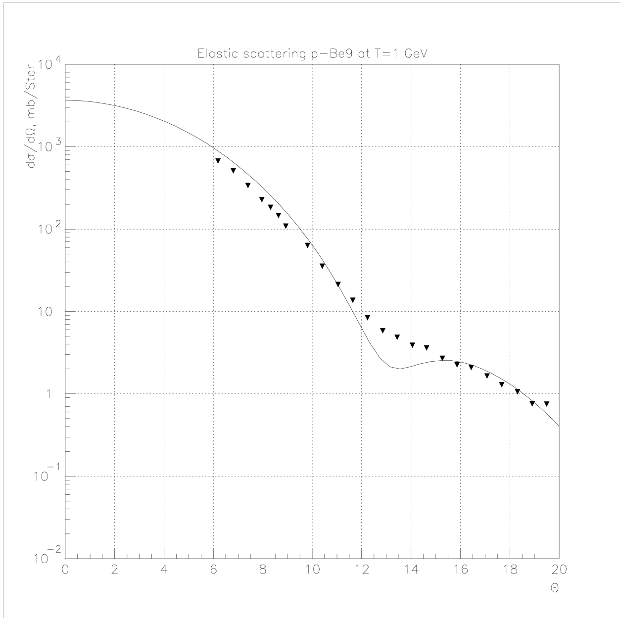
Fig. 21.1: Elastic proton scattering on {}^9\text{Be} at 1 GeV.
