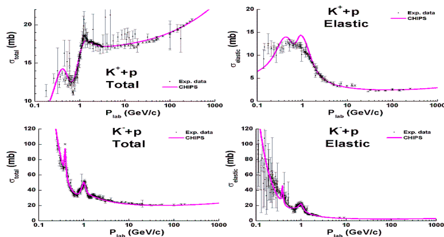
Fig. 23.7: Total and elastic cross sections of Kp -interactions. Points are experimental data from PDG data-base .
