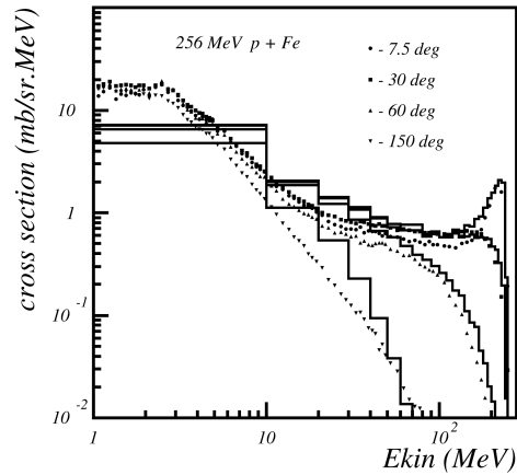
Fig. 25.6: Double differential cross-section for neutrons produced in proton scattering off Iron. Proton incident energy was 256 MeV. The points are data, the histogram is Binary Cascade prediction.
