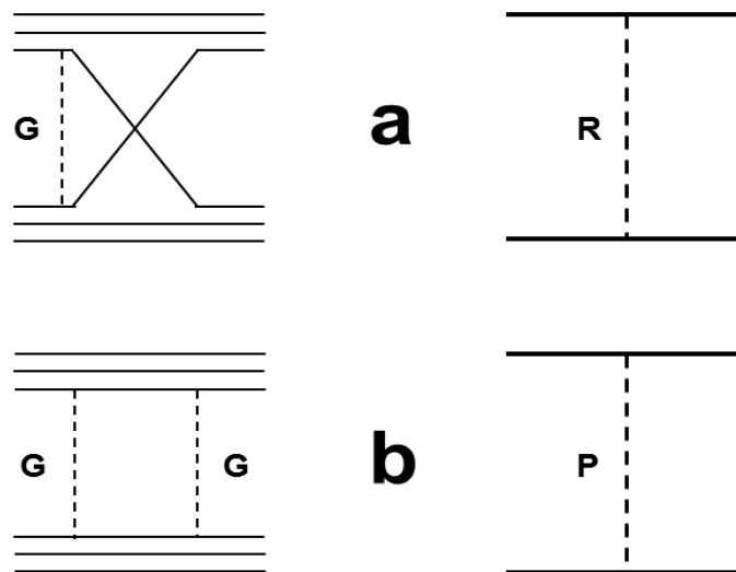
Fig. 23.20: Diagrams of quark-gluon exchanges and corresponding reggeon diagrams for hadron-nucleus interactions.
