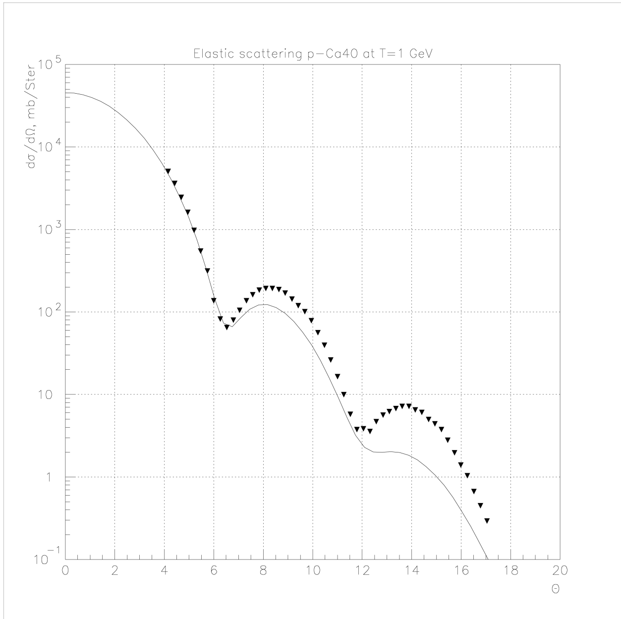
Fig. 21.6: Elastic proton scattering on ^{40}\text{Ca} at 1 GeV.
