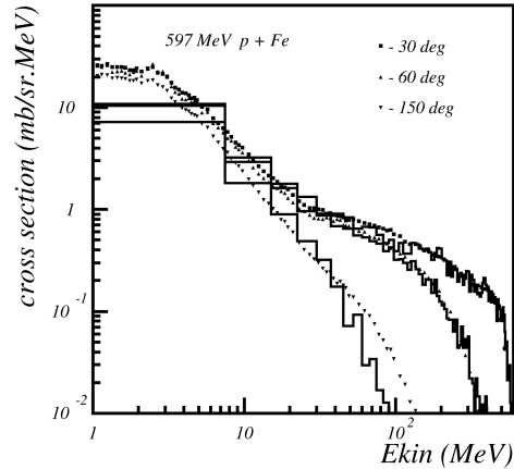
Fig. 25.7: Double differential cross-section for neutrons produced in proton scattering off Iron. Proton incident energy was 597 MeV. The points are data, the histogram is Binary Cascade prediction.
