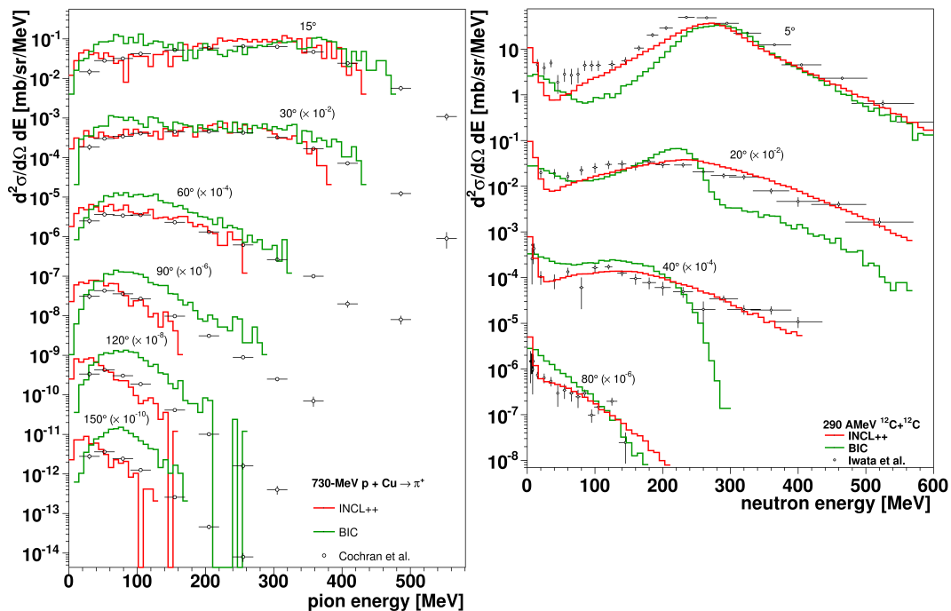
Fig. 26.2: Left: double-differential cross sections for the production of charged pions in 730-MeV p + \text{Cu} . Right: double-differential cross sections for the production of neutrons in 290-AMeV ^{12}\text{C} + ^{12}\text{C} . Predictions of the INCL++ and Binary-Cascade models are compared with experimental data from Refs. [CDG+72] and [IMS+01].
