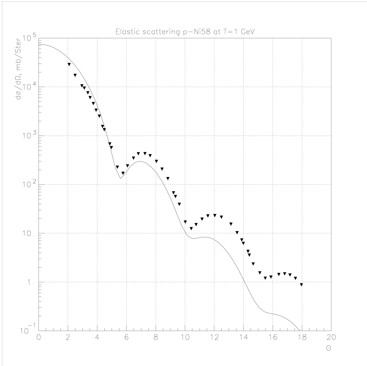
Fig. 21.7: Elastic proton scattering on ^{58}\text{Ni} at 1 GeV.
