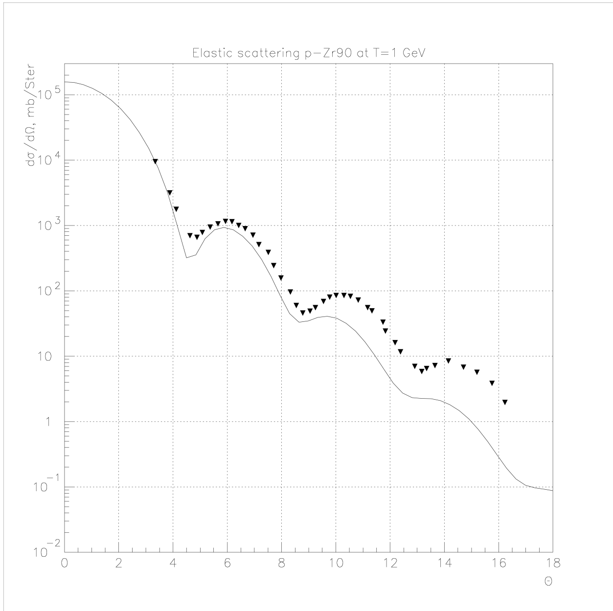
Fig. 21.8: Elastic proton scattering on ^{90}\text{Zr} at 1 GeV.
