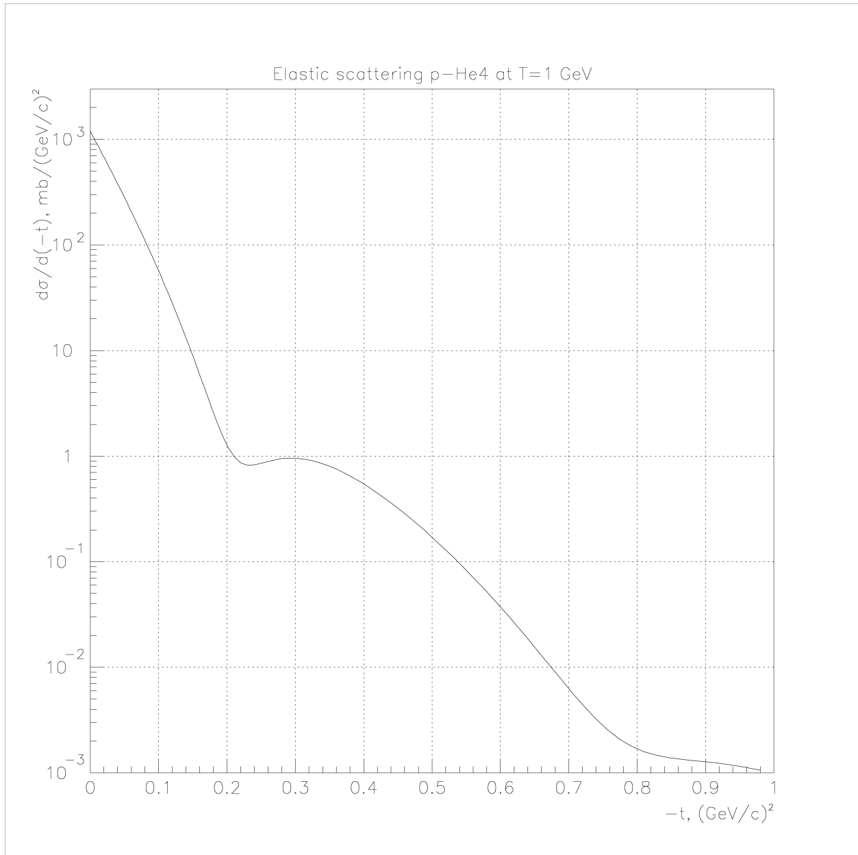
Fig. 21.10: Elastic proton scattering on 4 He at 1 GeV.
