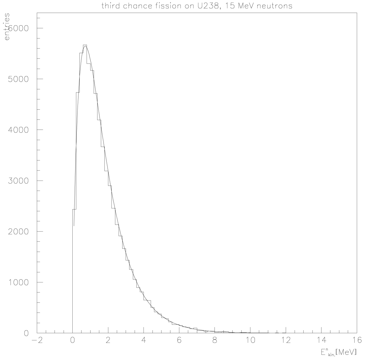
Fig. 37.3: Comparison of data and Monte Carlo for fission neutron energy distributions for induced fission by 15 MeV neutrons on uranium ( ^{238}\text{U} ). The curve represents evaluated data and the histogram is the Monte Carlo prediction.
