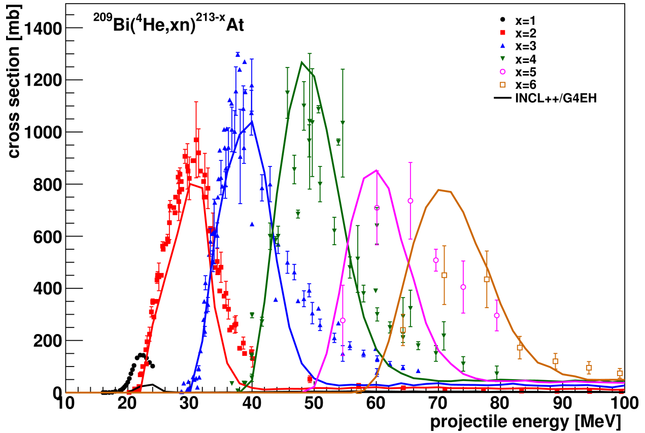
Fig. 26.3: Excitation functions for (\alpha, xn) cross sections on ^{209}\text{Bi} . The predictions of INCL++-G4ExcitationHandler are represented by the solid line and are compared to experimental data [BL74, DL74, eal05, KSegre49, LM85, RBAC90, SMS94, SH74, PatelShahSingh99].
