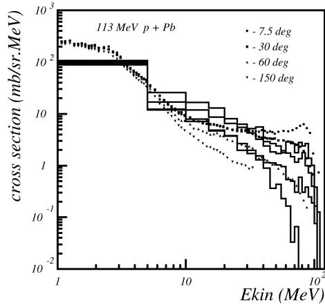
Fig. 25.9: Double differential cross-section for neutrons produced in proton scattering off Lead. Proton incident energy was 113 MeV. The points are data, the histogram is Binary Cascade prediction.
