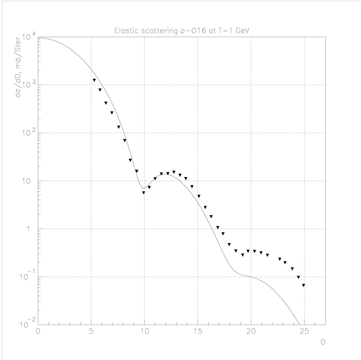
Fig. 21.4: Elastic proton scattering on 16 O at 1 GeV.
