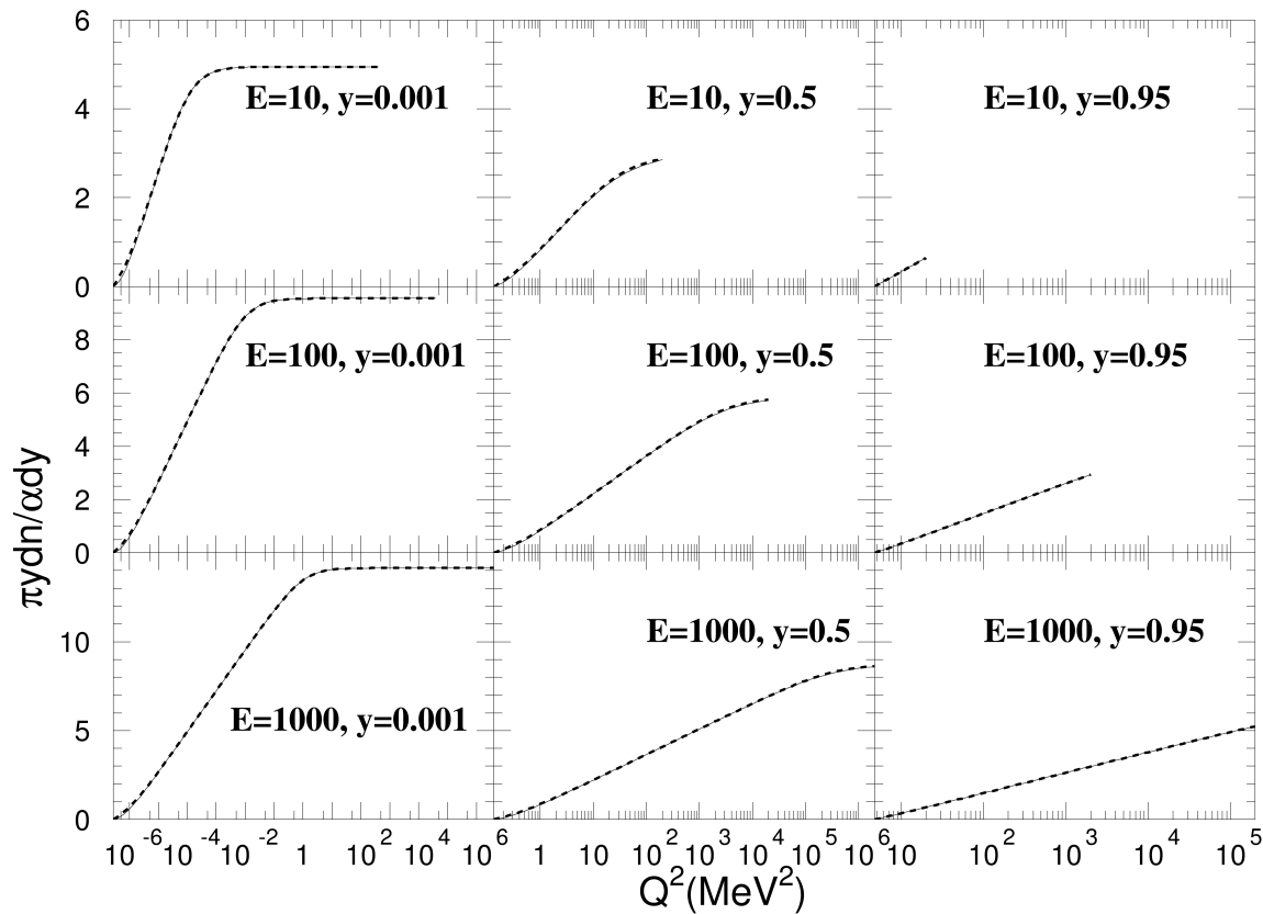
Fig. 42.2: Integrals of Q^2 spectra of virtual photons for three energies 10 MeV, 100 MeV, and 1 GeV at y=0.001 , y=0.5 , and y=0.95 . The solid line corresponds to Eq. (42.3) and the dashed line (which almost everywhere coincides with the solid line) corresponds to Eq. (42.8).
