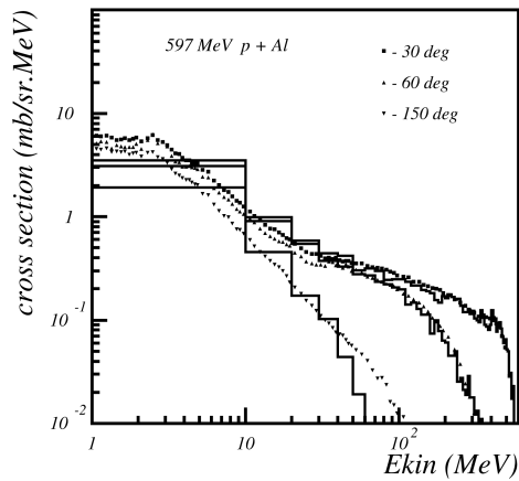
Fig. 25.3: Double differential cross-section for neutrons produced in proton scattering off Aluminum. Proton incident energy was 597 MeV. The points are data, the histogram is Binary Cascade prediction.
