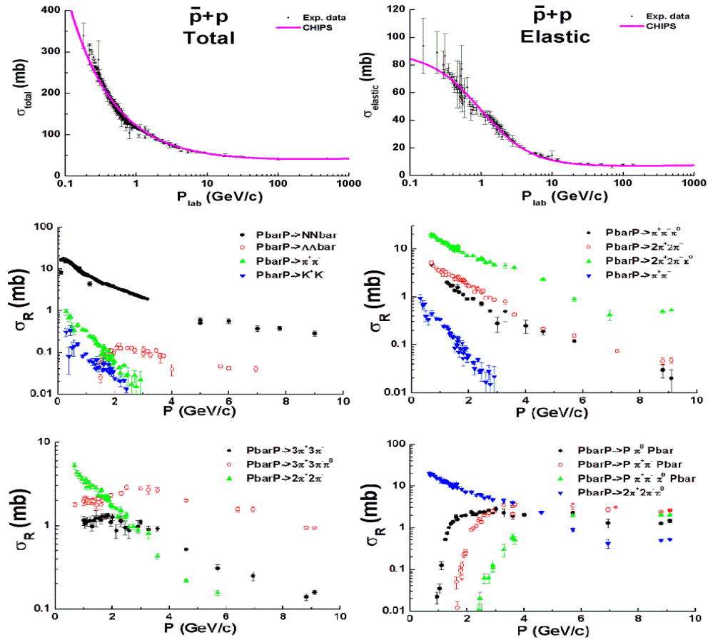
Fig. 23.9: General properties of \bar{p}p -interactions. Points are experimental data: data on total and elastic cross sections from PDG data-base [PDG12], other data from [eal73a, eal84].
