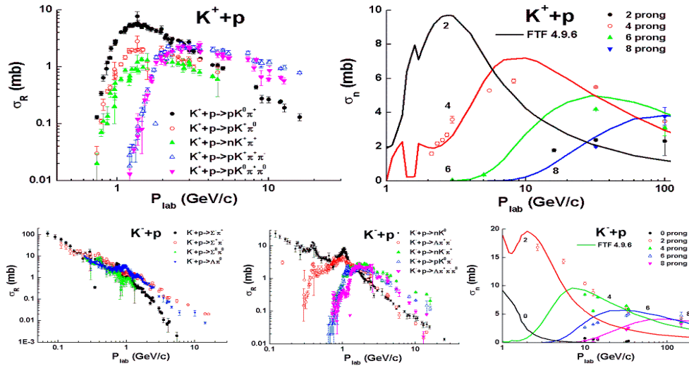
Fig. 23.8: Reaction cross sections of Kp -interactions. Points are experimental data.
