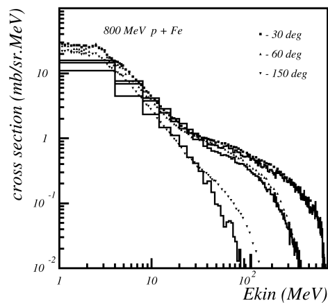
Fig. 25.8: Double differential cross-section for neutrons produced in proton scattering off Iron. Proton incident energy was 800 MeV. The points are data, the histogram is Binary Cascade prediction.
