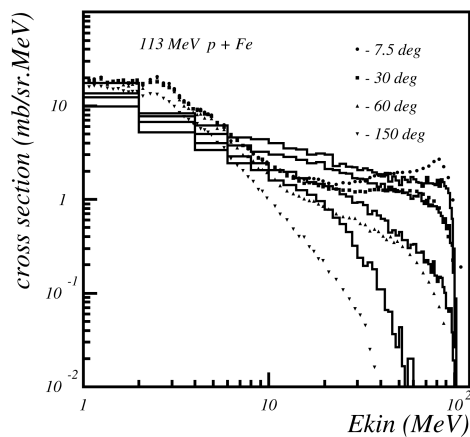
Fig. 25.5: Double differential cross-section for neutrons produced in proton scattering off Iron. Proton incident energy was 113 MeV. The points are data, the histogram is Binary Cascade prediction.
