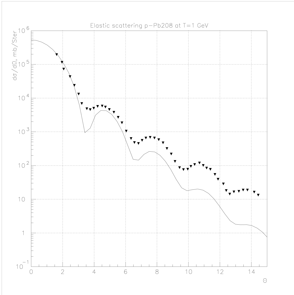
Fig. 21.9: Elastic proton scattering on ^{208}\text{Pb} at 1 GeV.
