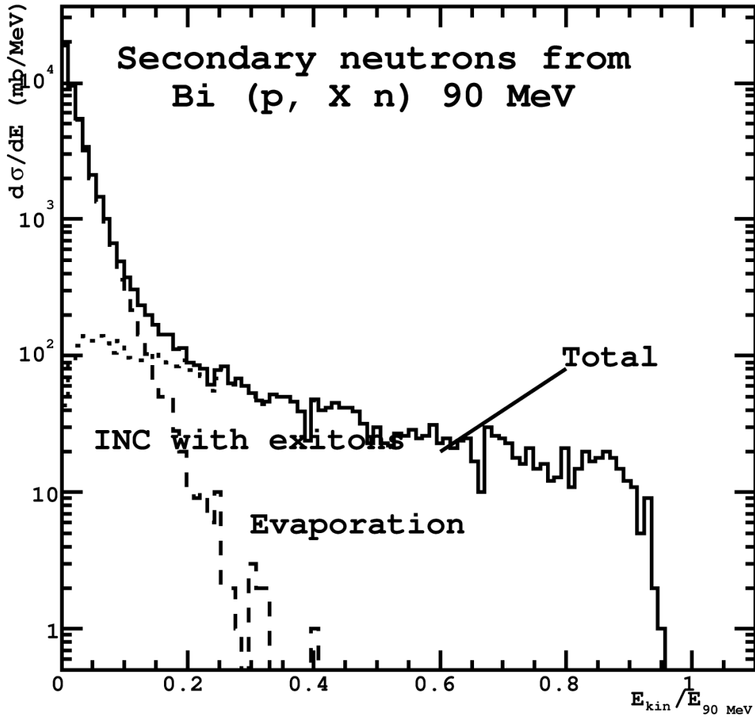
Fig. 24.1: Secondary neutrons generated by Bertini INC with excitons and evaporation model.
