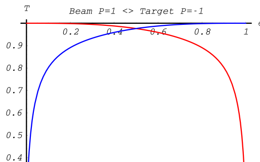
Fig. 13.9: Polarization transfer functions in Møller scattering. Longitudinal polarization \xi_3^{(2)} of electron with energy E_{p_2} in blue; longitudinal polarization \xi_3^{(1)} of second electron in red. Kinetic energy of incoming electron T_{k_1} = 10\text{MeV}
