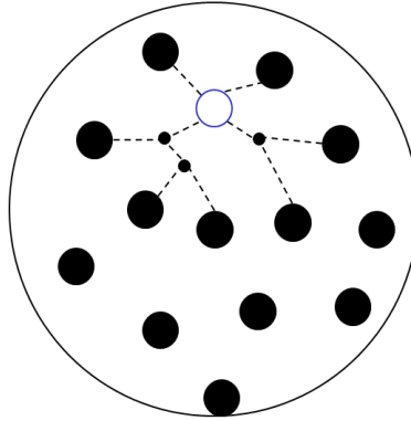
Fig. 23.19: Reggeon “cascade” in hA -scattering.
