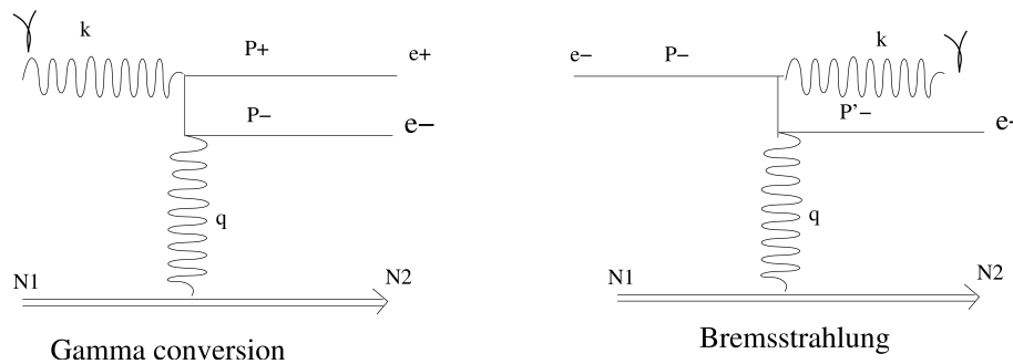
Fig. 13.24: Feynman diagrams of Gamma conversion and bremsstrahlung processes.
