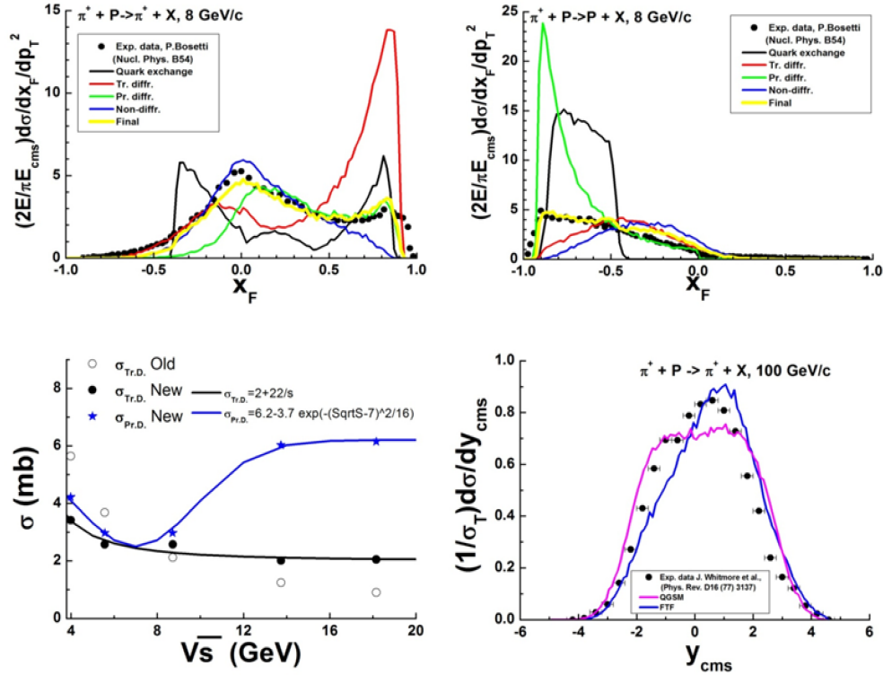
Fig. 23.12: Upper figures: inclusive spectra of protons and \pi^+ -mesons in \pi^+p -interactions. Points are experimental data [eal73b]. Lines represent the contributions of the various FTF processes calculated by assuming that the probability of each process is 100 %. Bottom left figure: diffraction dissociation cross sections obtained by tuning (points), and their description (lines) by the expression for \pi in (23.4). Bottom right figure: rapidity spectrum of \pi^+ -mesons in \pi^+p -interactions at p_{lab} = 100 GeV/c. Points are experimental data [Whi74].
