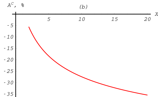
Fig. 13.19: Compton total cross section asymmetry depending on the energy of incoming photon. Up to 10MeV.
