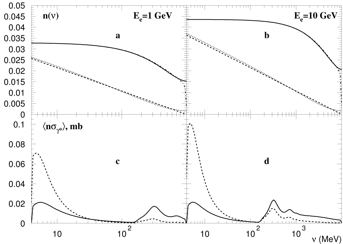
Fig. 42.1: Relative contribution of equivalent photons with small Q^2 to the total “photon flux” for (a) 1 GeV electrons and (b) 10 GeV electrons. In figures (c) and (d) the equivalent photon distribution dn(\nu, Q^2) is multiplied by the photonuclear cross section \sigma_{\gamma^*}(K, Q^2) and integrated over Q^2 in two regions: the dashed lines are integrals over the low- Q^2 equivalent photons (under the dashed line in the first two figures), and the solid lines are integrals over the high- Q^2 equivalent photons (above the dashed lines in the first two figures).
