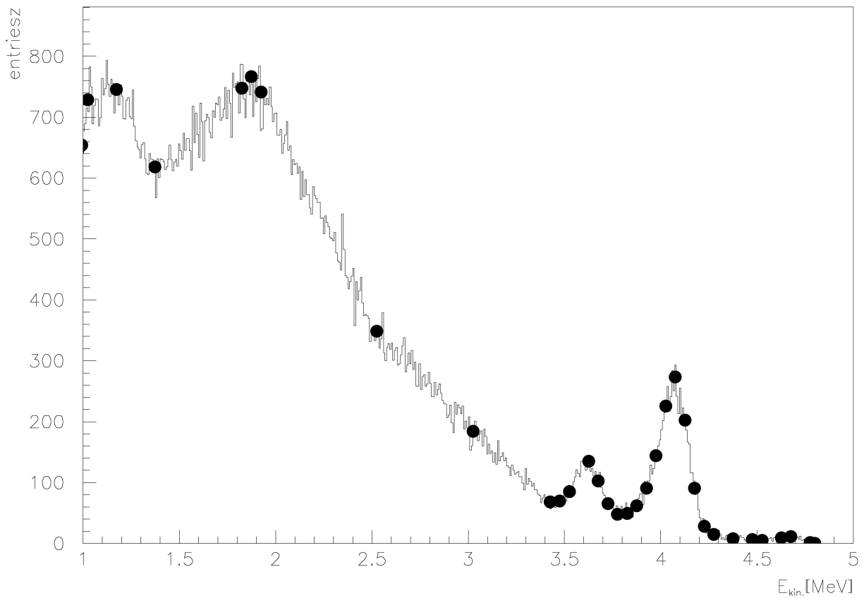
Fig. 37.2: Comparison of data and Monte Carlo for photon energy distributions for radiative capture of 15 MeV neutrons on Uranium ( ^{238}\text{U} ). The points are evaluated data, the histogram is the Monte Carlo prediction. 385
