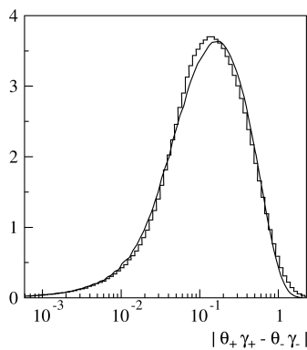
Fig. 6.15: Distribution of the difference of transverse momenta of positive and negative muons (with logarithmic x-scale).
