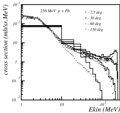
Fig. 25.10: Double differential cross-section for neutrons produced in proton scattering off Lead. Proton incident energy was 256 MeV. The points are data, the histogram is Binary Cascade prediction.
