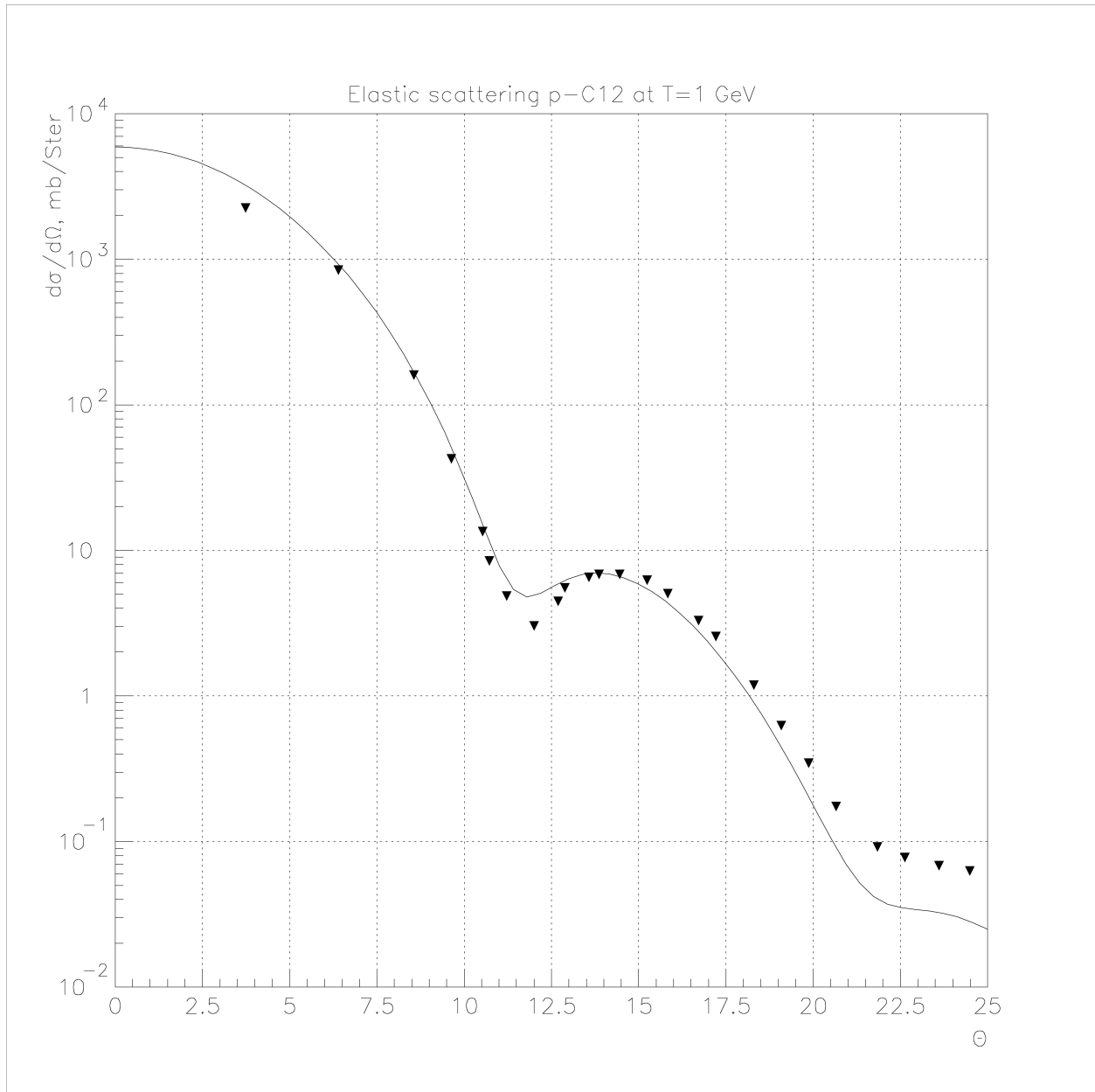
Fig. 21.3: Elastic proton scattering on ^{12}\text{C} at 1 GeV.
