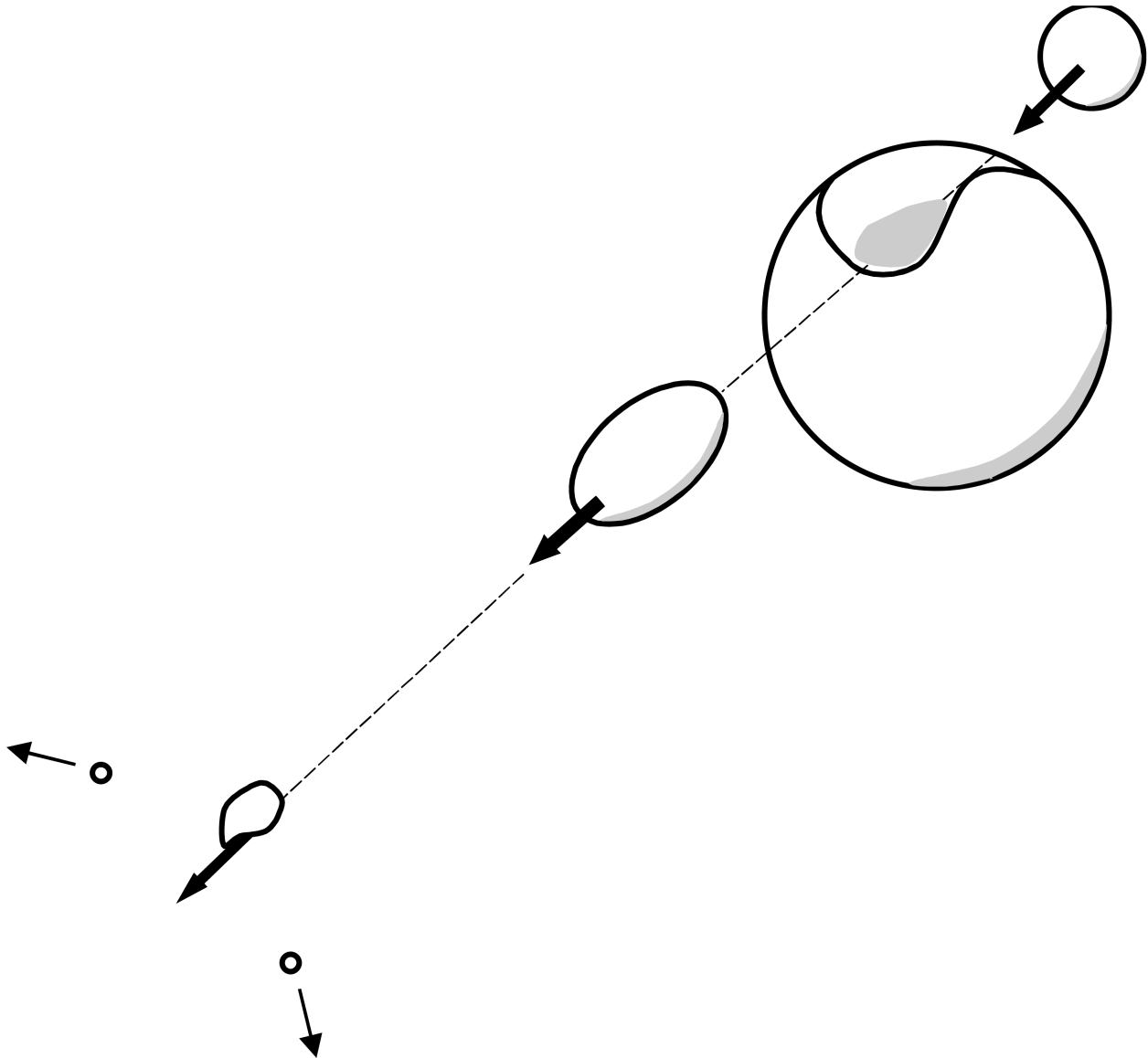
Fig. 34.1: In the abrasion process, a fraction of the nucleons in the projectile and target nucleons interact to form a fireball region with a velocity between that of the projectile and the target. The remaining spectator nucleons in the projectile and target are not initially affected (although they do suffer change as a result of longer-term de-excitation).
