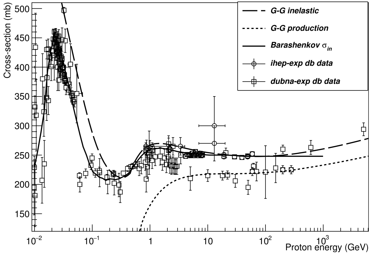
Fig. 19.2: Inelastic and production cross-sections of protons on a carbon target in the energy range 10^{-2} - 10^3 GeV. Experimental data (open points and squares) are from [IHEP, NEA]. The solid and dashed lines correspond to the Barashenkov and Glauber-Gribov inelastic models, respectively. The dotted line shows the Glauber-Gribov production model.
