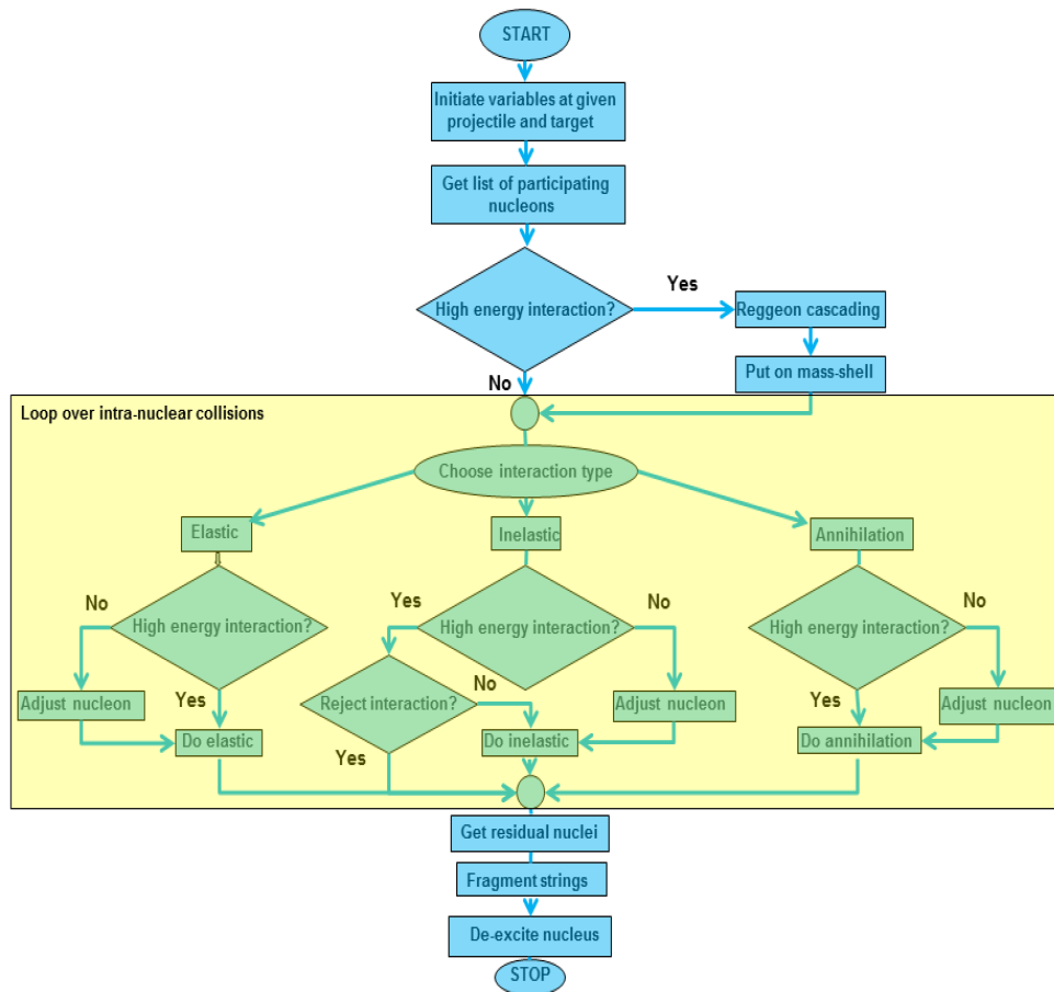
Fig. 23.14: Flowchart of the FTF model.
