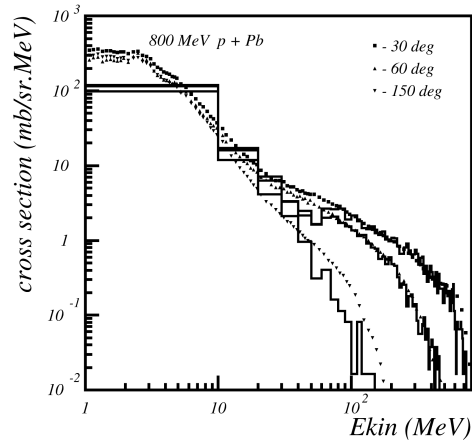
Fig. 25.12: Double differential cross-section for neutrons produced in proton scattering off Lead. Proton incident energy was 800 MeV. The points are data, the histogram is Binary Cascade prediction.
