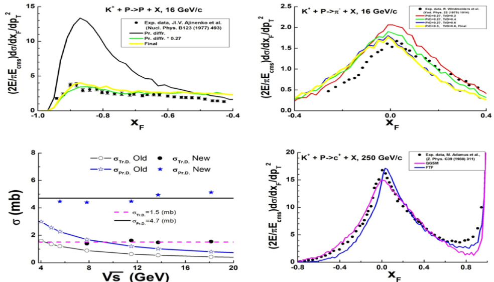
Fig. 23.13: Upper figures: inclusive spectra of protons and \pi^- -mesons in Kp^* -interactions. Points are experimental data* :cite:had-Ajinenko,had-Ajinenko2. Lines are FTF calculations. Bottom left figure: diffraction dissociation cross sections obtained by tuning (points), and their description (lines) by the expression for Kp in (23.4). Bottom right figure: x_F spectrum of positive charged particles in Kp -interactions at p_{lab} = 250 GeV/c. Points are experimental data [Whi74], lines are model calculations.
