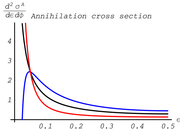
Fig. 13.14: Annihilation differential cross section in arbitrary units. Black line corresponds to unpolarized cross section; red line – to the antiparallel spins of initial particles, and blue line – to the parallel spins. Kinetic energy of the incoming positron T_{k_1} = 10\text{MeV} .
