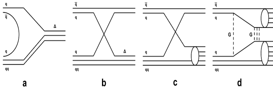
Fig. 23.4: Quark flow diagrams of \pi N -interactions.
