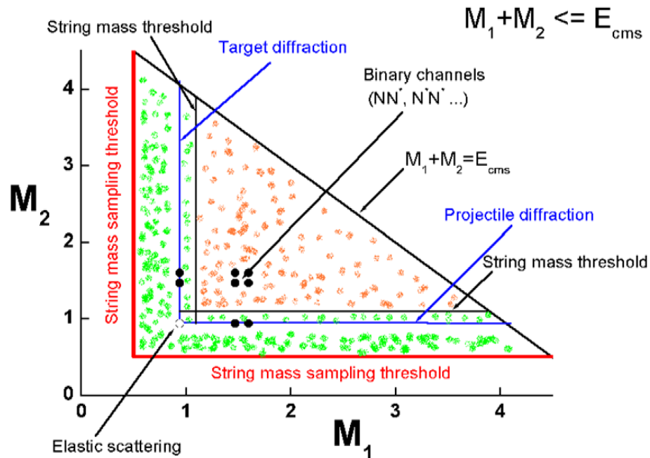
Fig. 23.2: Diagram of the final states of hadron-hadron interactions.
