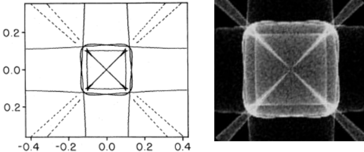
Fig. 47.1: Left: outline of phonon caustics in germanium as predicted by Northrop and Wolfe [NW79]. Right: Phonon caustics as simulated using the GEANT4 phonon transport code.
